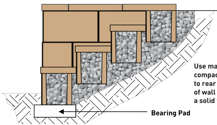
CROSS SECTION
